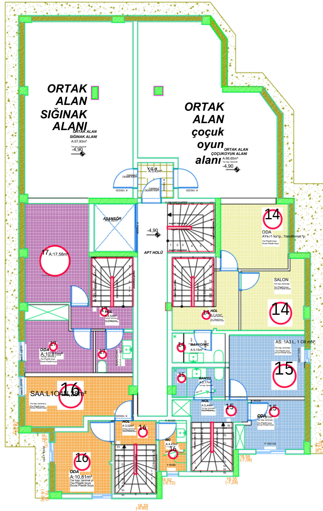
-2. BODRUM KAT PLANI
